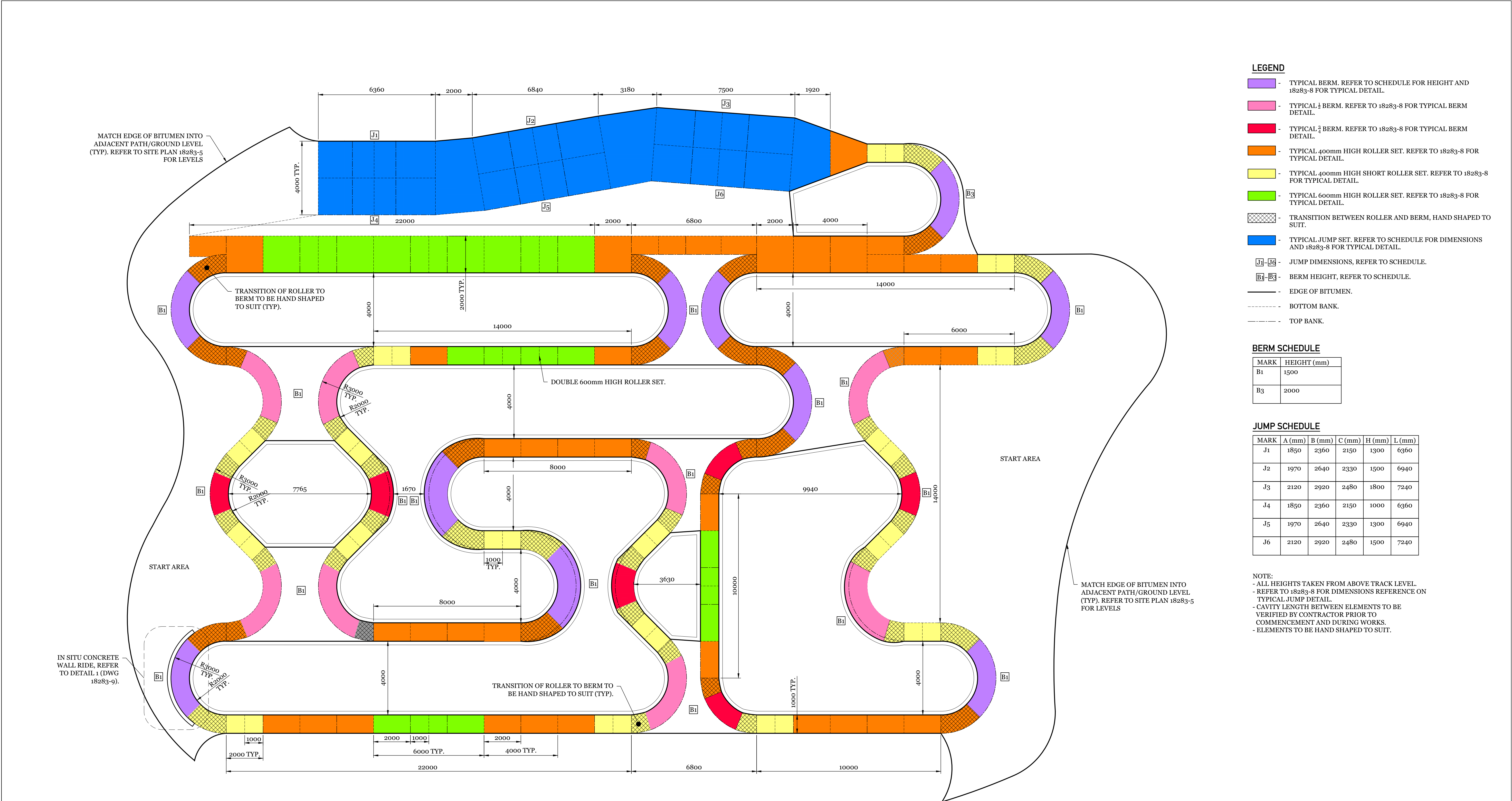
LAYOUT PLAN - INTERMEDIATE PUMP TRACK SCALE 1:100
